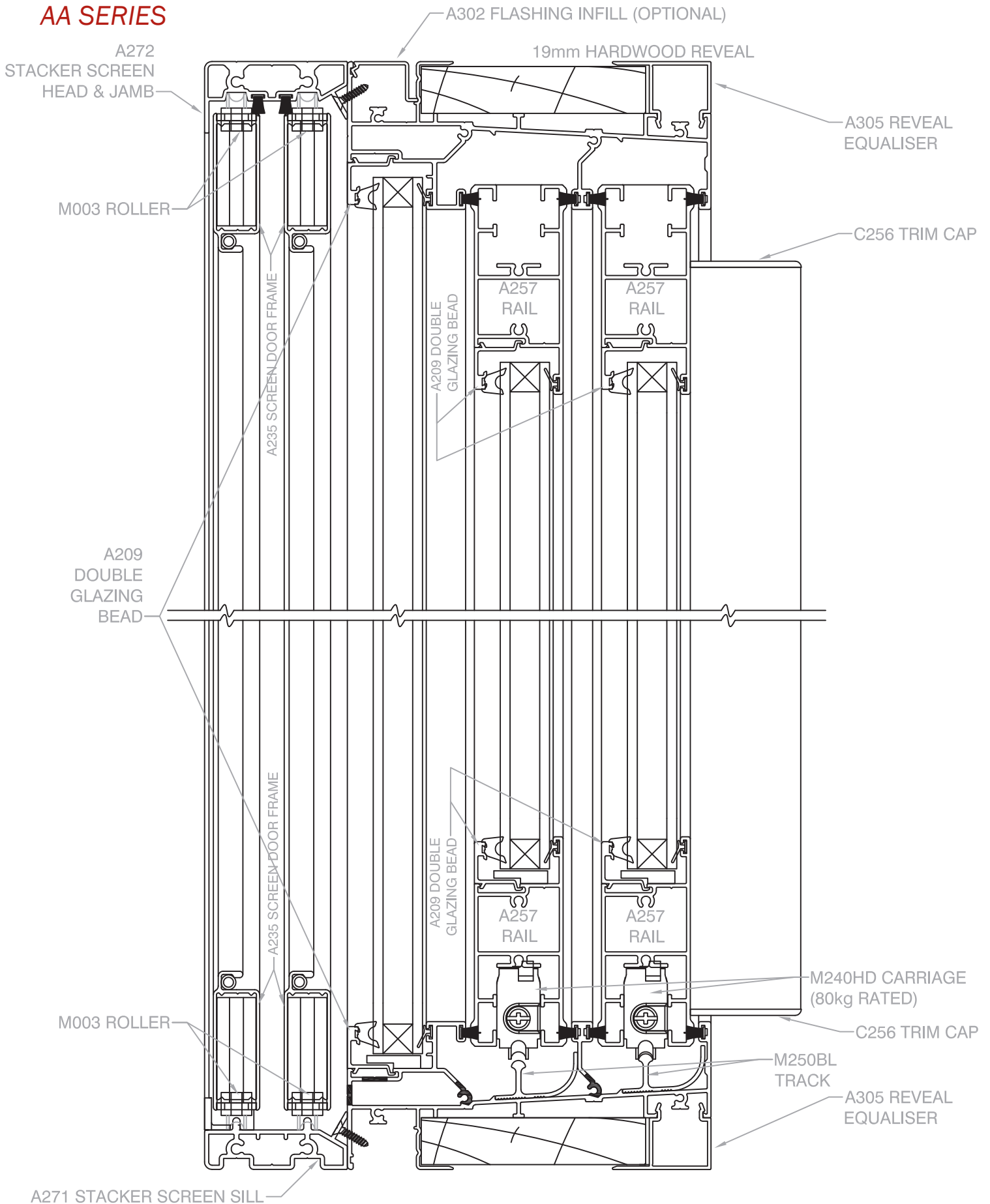
Scale 1 : 2 @ A4, Vertical Cross Section illustrating A305 reveal equaliser
