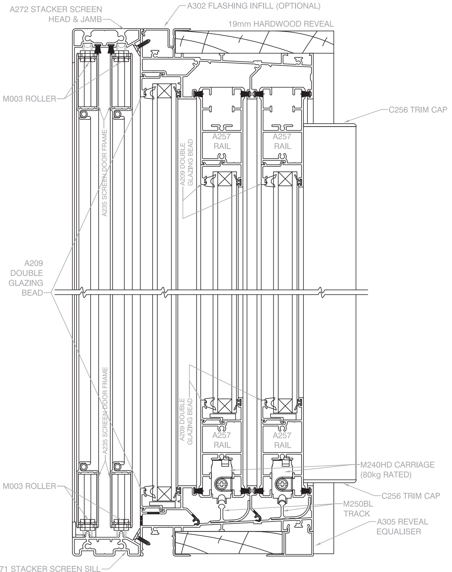
Scale 1 : 2 @ A4, Vertical Cross Section
