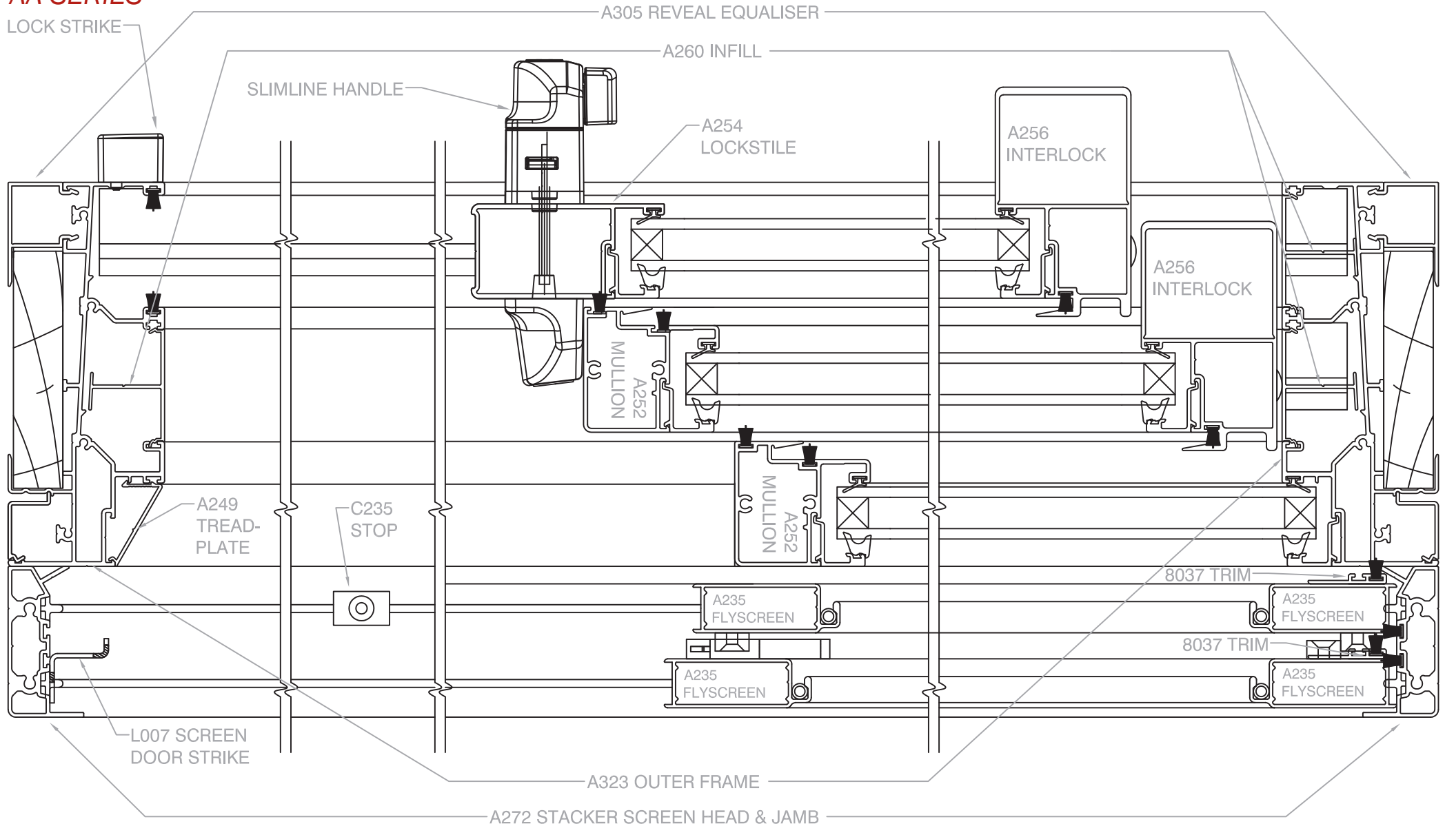
Scale 1 : 2 @ A4, Horizontal Cross Section of 3-Panel Stacker Door illustrating A305 reveal equaliser
