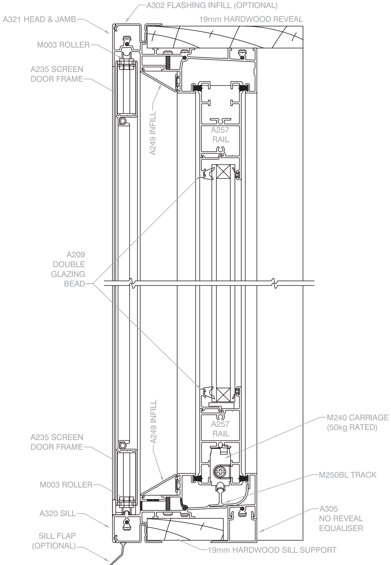
Scale 1 : 2 @ A4, Vertical Cross Section of 2 Panel - 2 Panel Corner Sliding Door
